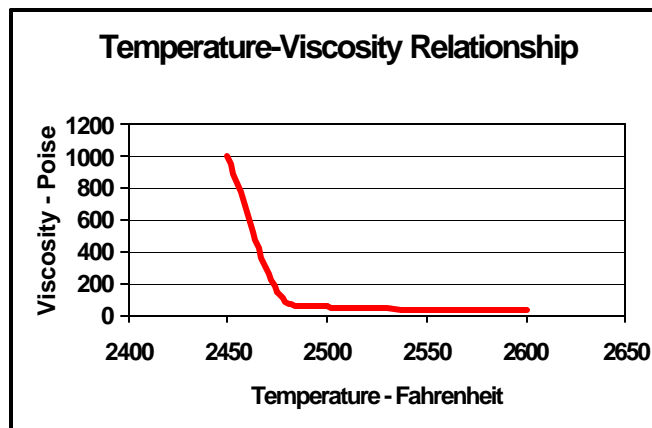
Ash Viscosity Measurement
